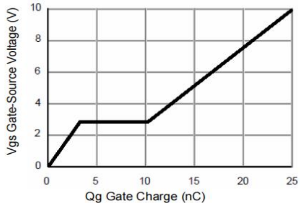
Figure 6: Gate-Charge Characteristics
