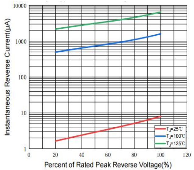
Figure 4: Reverse Characteristics
