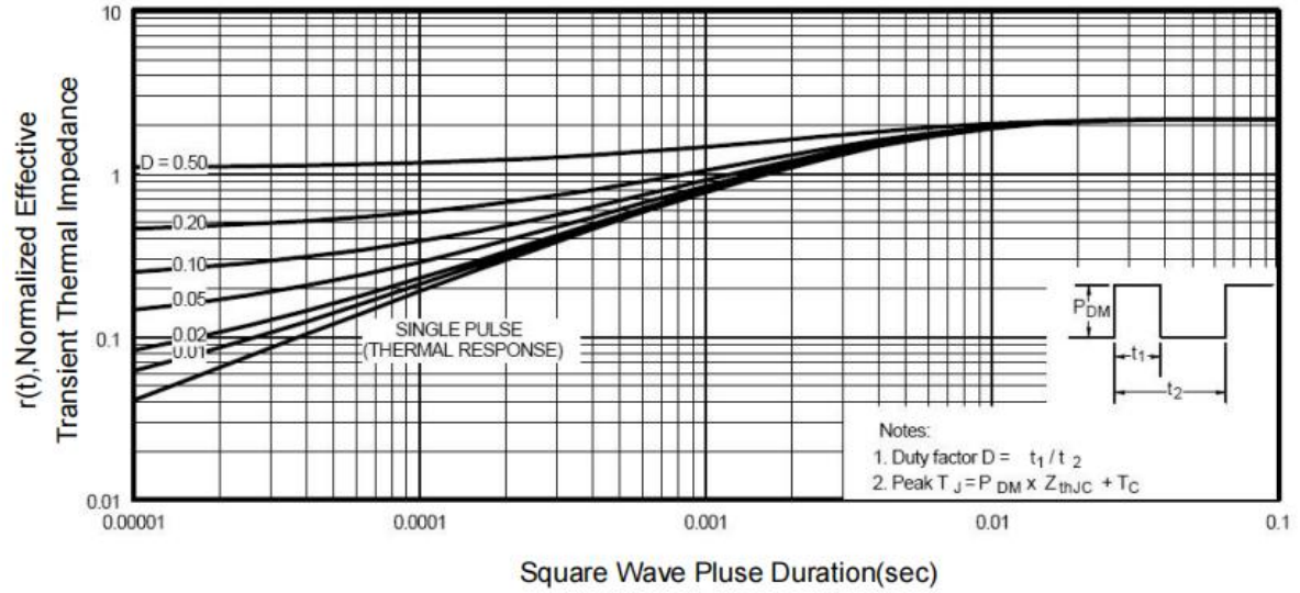
Figure 9: Transient Thermal Response Curve
