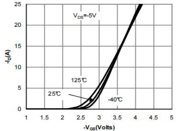
Figure 4: Transfer Characteristics
