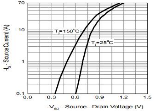
Figure 2: Diode Characteristics
