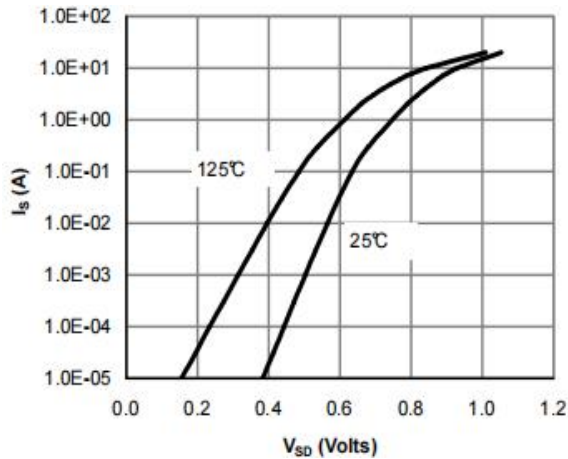
Figure 9: Diode Characteristics
