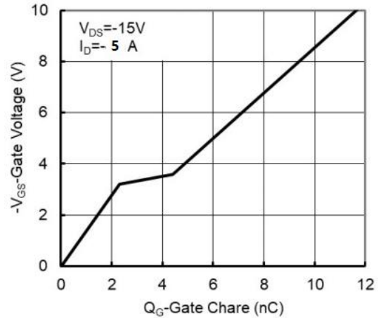
Figure 6: Gate-Charge Characteristics
