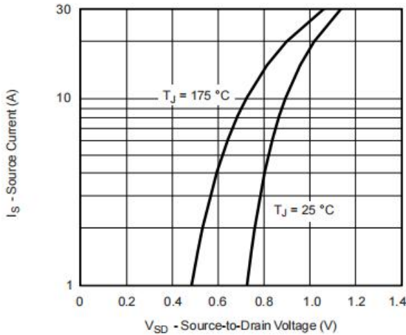
Figure 7: Diode Characteristics
