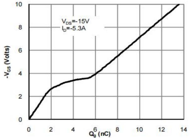
Figure 6: Gate-Charge Characteristics
