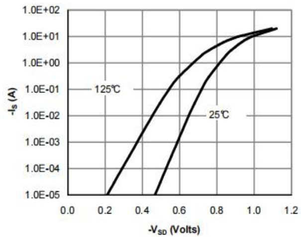
Figure 7: Diode Characteristics
