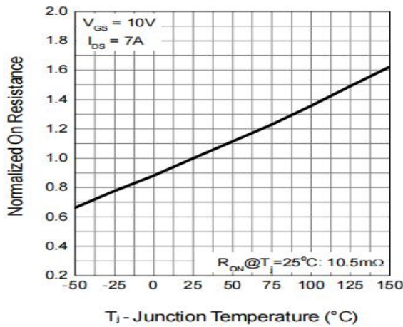
T J - Junction Temperature (°C)
