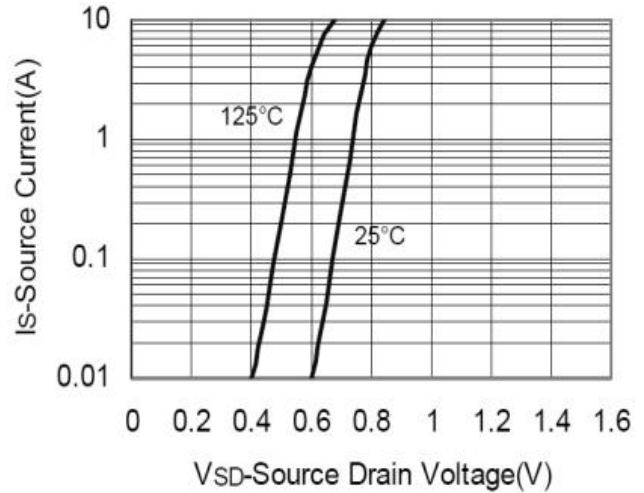
Figure 8: Diode Characteristics
