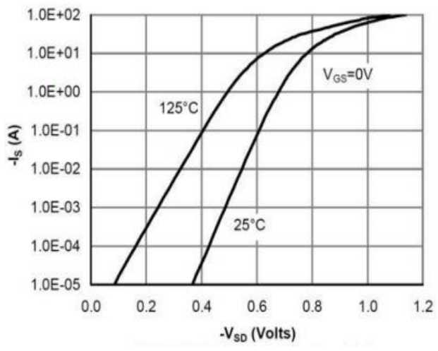
Figure 8: Diode Characteristics
