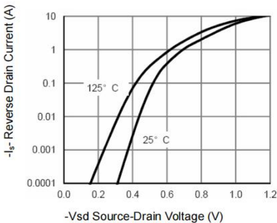
Figure 9: Diode Characteristics
