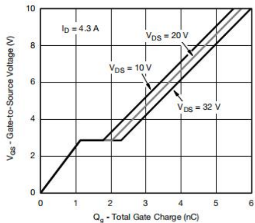
Figure 6: Gate-Charge Characteristics
