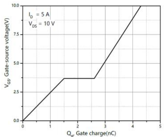
Figure 6: Gate-Charge Characteristics
