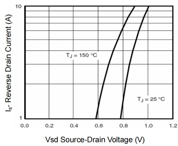
Figure 7: Diode Characteristics
