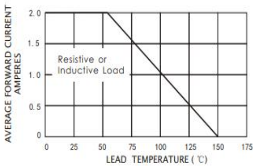
Figure 1: Forward Current Curve
