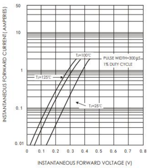
Figure 3: Forward Characteristics
