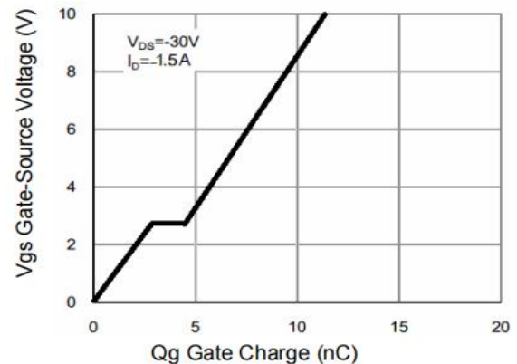
Figure 6: Gate-Charge Characteristics
