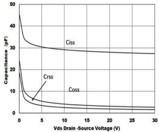
Figure 4: Capacitance Characteristics
