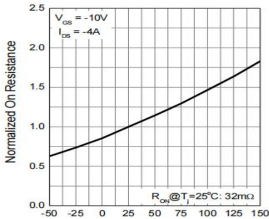
T_J - Junction Temperature ( ^{\circ}\text{C} )
