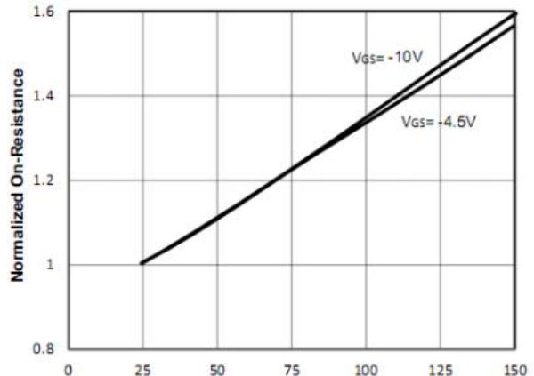
T_J Junction Temperature ( ^\circ\text{C} ) Figure 4: On-Resistance vs. Temperature
