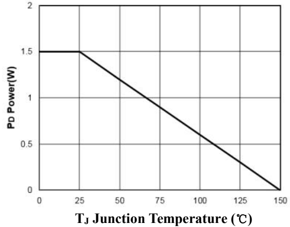
Figure 8: Power Dissipation
